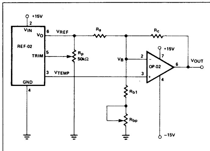
Figure 2. Complete Schematic
